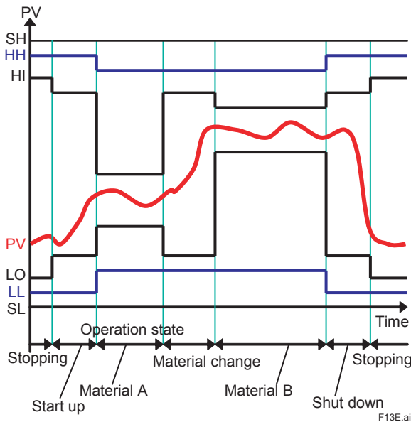
Figure Dynamic Alarm Threshold Setting Function
