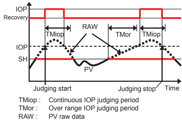
Figure Judging of IOP/IOP- Alarms (Over range)
