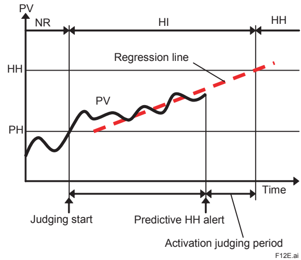
Figure Predictive HH/LL Alert
