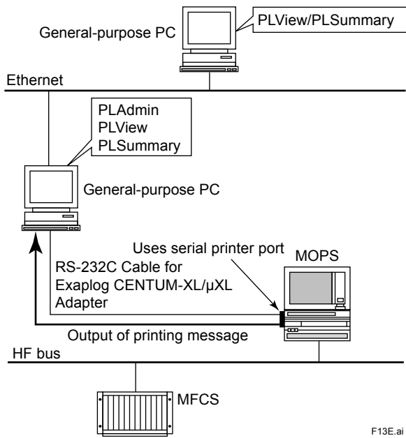
Figure: μXL Connection Example
